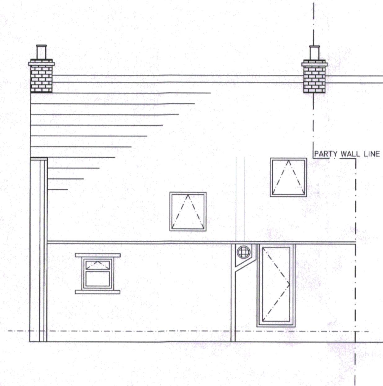
E ELEVATION EAST 1:50
